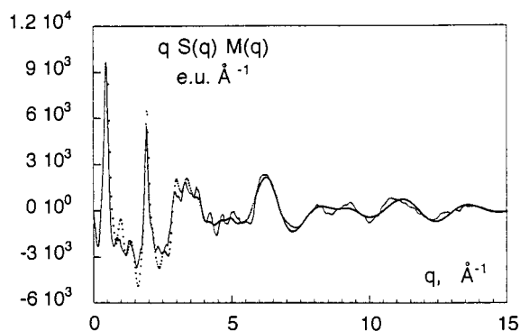
Figure 1. Observed (—) and calculated (···) qS(q)M(q) values vs q .
