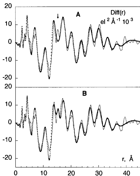
Figure 2. Experimental function \text{Diff}(r) = D(r) - 4\pi r^2 \rho_0 (—) and the theoretical calculated function (···), as illustrated in the text.
