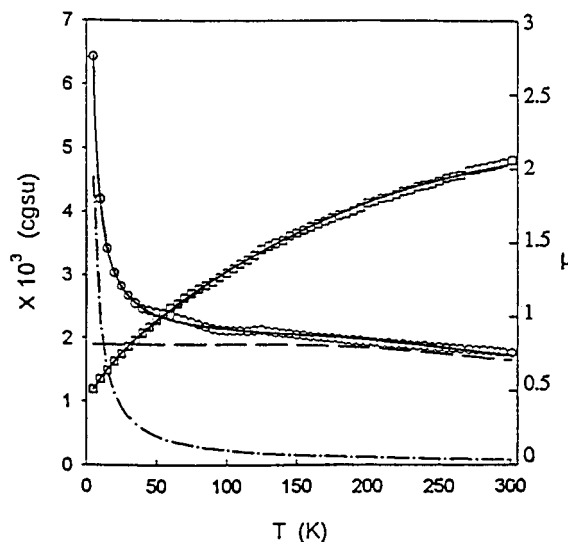
Figure 5. Temperature dependence of \chi'_M vs T (K) (exptl, \circ ; calcd, —; \chi_0 , - -; \chi_{\text{imp}} , - · -) and \mu vs T (exptl, \square ; calcd, —).
